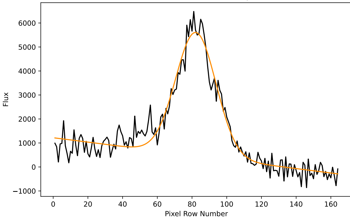
Column 871 Fit from Flux Calibrated J0800+3743
